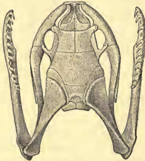
Skull of Chersydrus granulatus .
